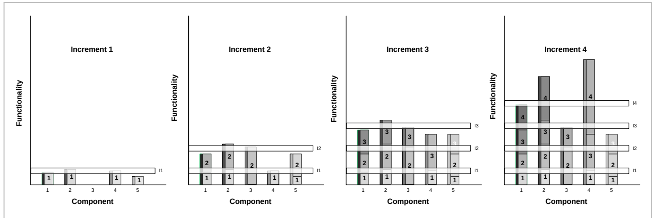
Figure 2: Agile/Incremental Build
